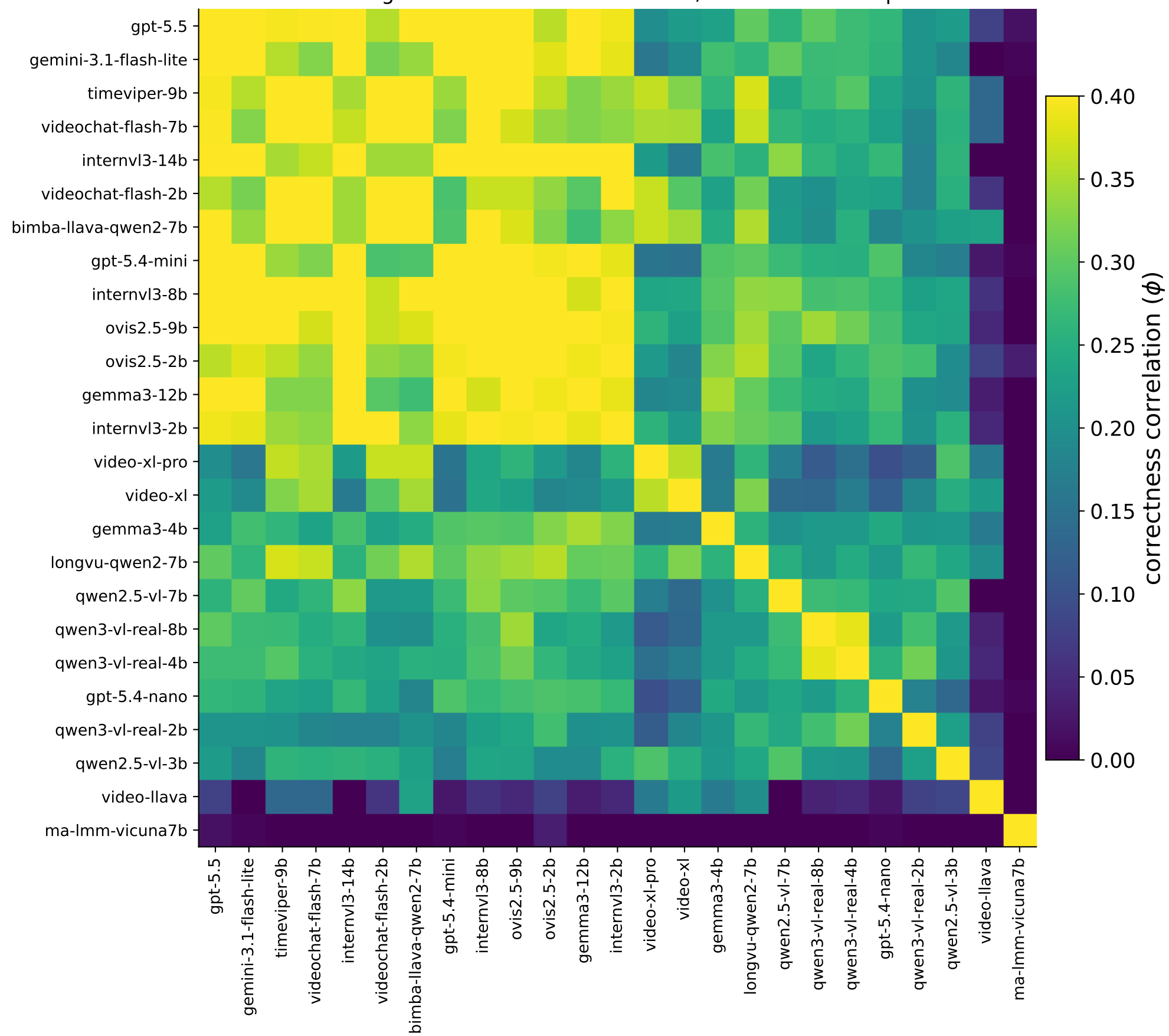
Inter-model agreement: do models succeed/fail on the same questions?
