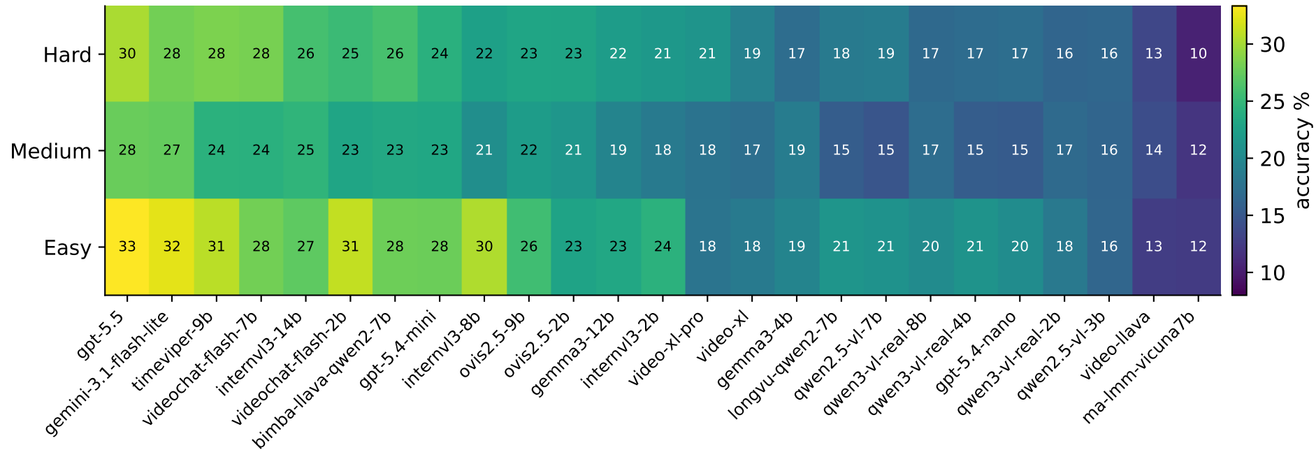
Accuracy by difficulty
