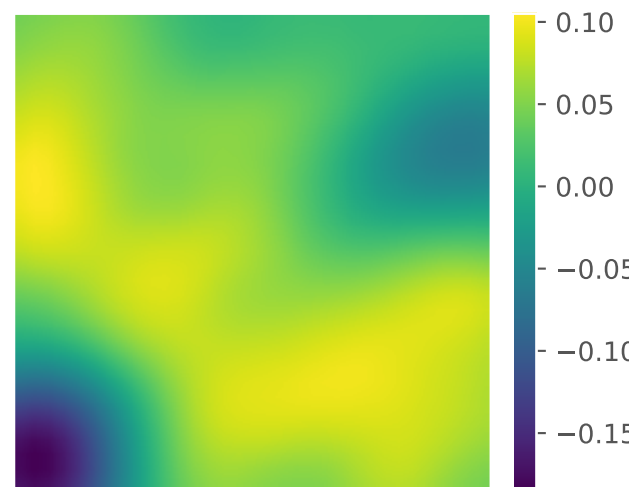
h-MALA Mean
