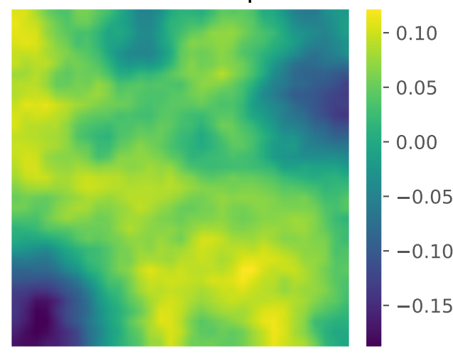
h-MALA Sample
