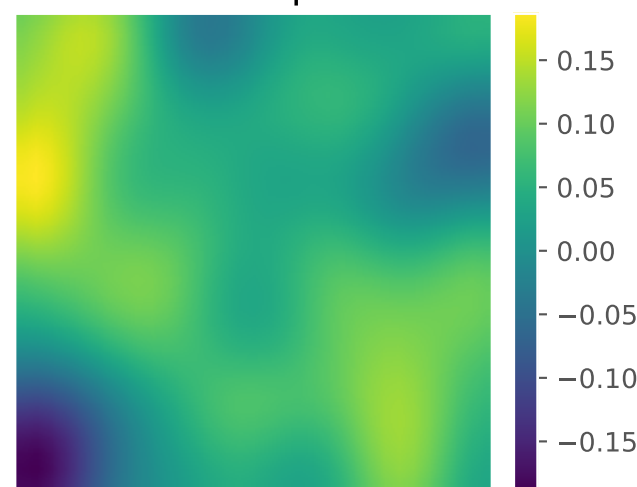
h-MALA Sample
