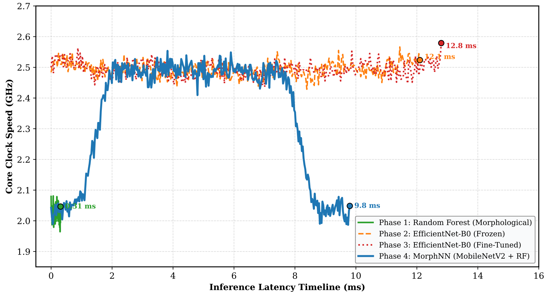
CPU Core Frequency During Inference
