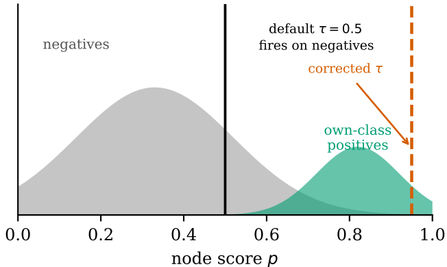
RFOED-NN: over-confident (training-prior / threshold mismatch)
