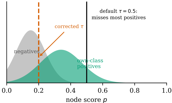
RFOED-RF: under-confident (test-time generalization gap)
