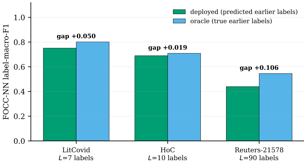
Exposure bias: the price of predicting earlier links is large on the 90-label chain, modest on the short ones
