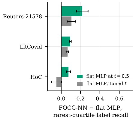
(c) multi-label: the chain's rare-label gain vs threshold
