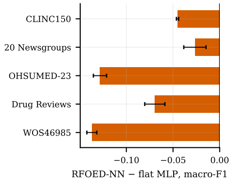
(b) single-label: the peel costs accuracy everywhere
