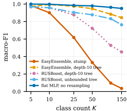
(a) the collapse is class count × weak-learner capacity
