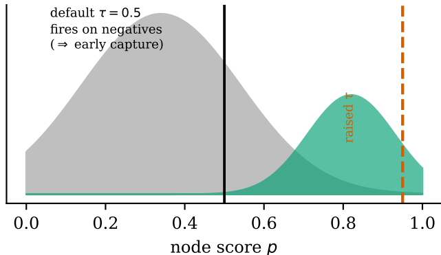
RFOED-NN: over-confident (training-prior / threshold mismatch)
