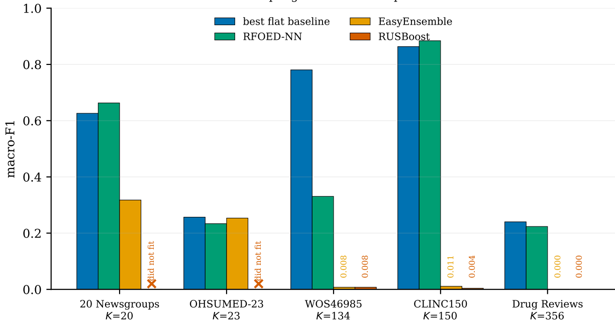
At native class count: resampling ensembles collapse or fail to fit once K > 100
