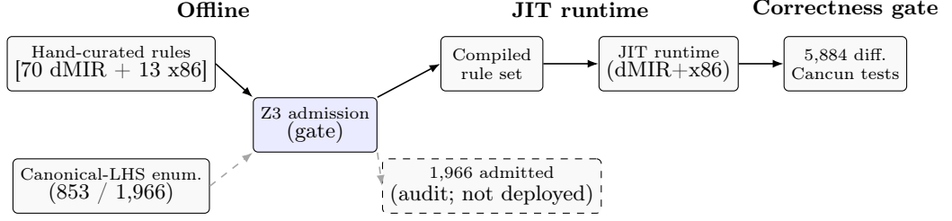
Fig. 2. Two-tier system overview. Hand-curated production rules ( 70 dMIR + 13 x86) pass an offline Z3 admission gate (admit rates: 98.7% algebraic, 21.8% carry-template) and become the compiled rule set deployed by the JIT (dMIR matcher followed by x86 CgIR cleanup); correctness is gated by 5,884 differential Cancun tests. In parallel, canonical-LHS enumeration submits 853 capacity-run candidates and produces 1,966 admitted rewrites whose canonical left-hand sides cover all 70 production rules; the audit channel (dashed) is a measurement output and is not deployed to the JIT.
