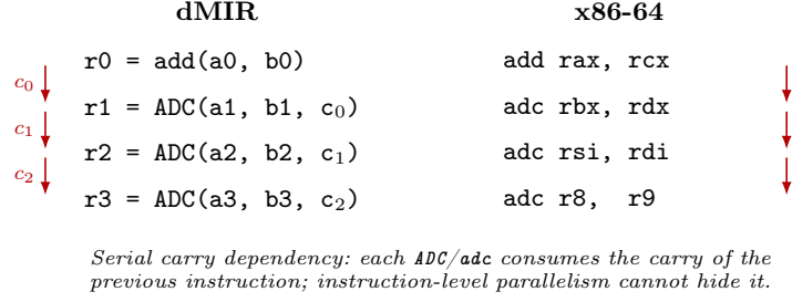
Fig. 1. U256 4-limb addition lowered to dMIR (left) and x86-64 (right). The first instruction is an ordinary 64-bit add ; each subsequent ADC (dMIR) / adc (x86-64) consumes the carry output of the previous instruction (red arrows c_0, c_1, c_2 ), forming a strict serial data dependency.
