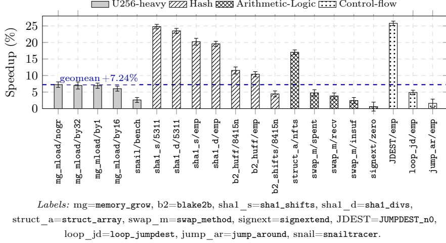
Fig. 3. Positive-speedup benchmark configurations from enabling the peephole rewrite rule set over the upstream-main baseline (error bars are 95% bootstrap confidence intervals, B=10\,000 ). The horizontal line at zero marks the no-change baseline; the dashed line at +7.24% marks the 27-benchmark geometric-mean speedup. From left to right, the benchmarks are grouped into four workload clusters: U256-heavy, Hash, Arithmetic-Logic, and Control-flow.
