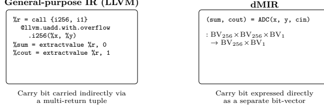
Fig. 1. Expressiveness comparison of general-purpose IR and dMIR on carry-propagating addition.
