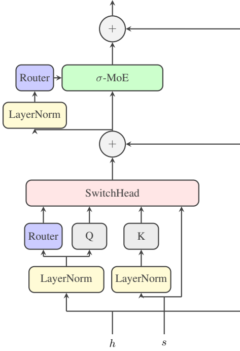
Figure 3: MoEUT Block. The original design was modified to account for the s that are attended to. They have their own LayerNorm and are passed as keys and values to the SwitchHead layer (instead of doing self-attention like in the original MoEUT).
