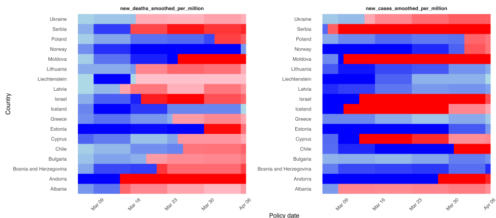
Figure 1: Outcome tensor from the merged OxCGRT–OWID panel. Rows are countries, columns are dates from March 5 to April 5, 2020, and panels are outcome–policy pairs. Outcomes are measured at a 28-day delay, so date t shows the value at t + 28 . Blue denotes policy-off entries, red policy-on entries, and darker shades larger outcome values.
