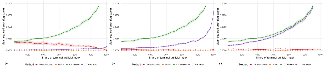
Figure 7: Castle masking experiment with additional missingness in the target layer k = 1 . The panels correspond to ranks r = 1, 2, 3 used for the four methods, with \tau = 0.01 for the tensor and matrix estimators. The terminal mask retains 9 fully observed rows and 4 fully observed columns. The curves report the average squared error over 10 replicates, with one standard error. The percentage on the x-axis represents the percentage of the terminal mask reached.
