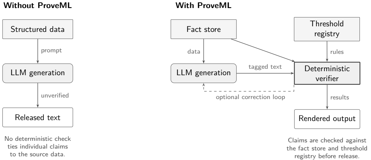
Figure 3: Without ProveML (left): data goes in, text comes out, no verification. With ProveML (right): every marked claim is checked against the fact store and threshold registry, with an optional correction loop. Rounded boxes denote generative components; squared boxes denote data stores and deterministic processing.
