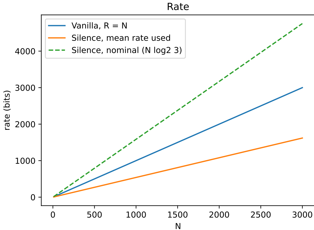
Vanilla vs. silence-is-free, ThresholdEncoder( t=[1.0] ) vs SilenceEncoder( t_{lo}=0.5, t_{hi}=2.0 ), SNR 0 dB
