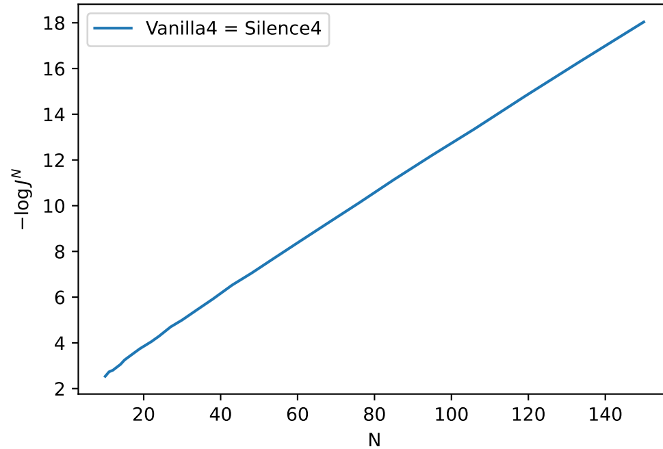
Total exponent (identical)
