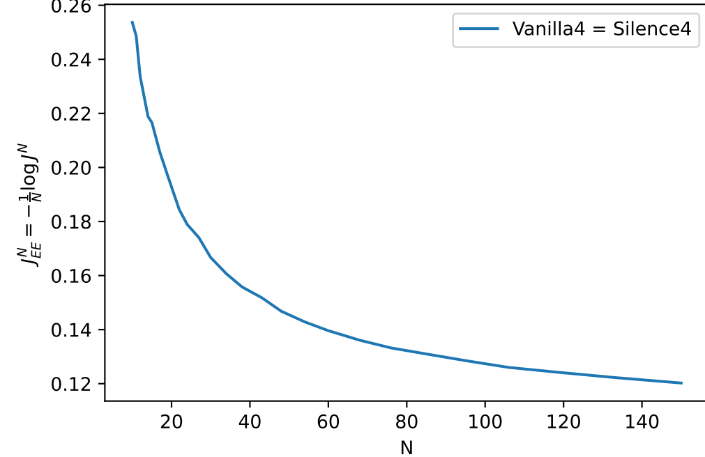
Normalized exponent (identical)
