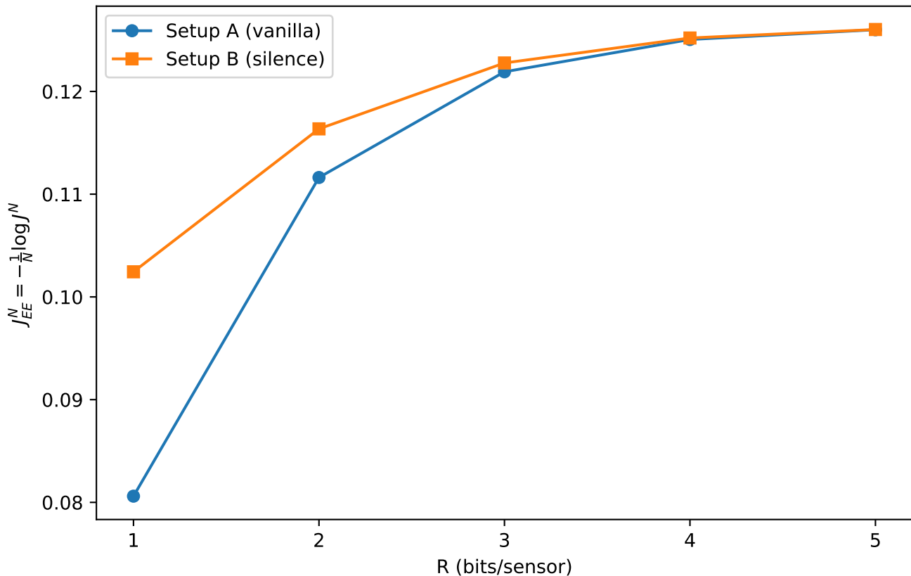
Normalized error exponent at optimal ( \Delta^* , \delta^* ) N=3000, SNR=0dB ( \mu=1 , \sigma=1 )
