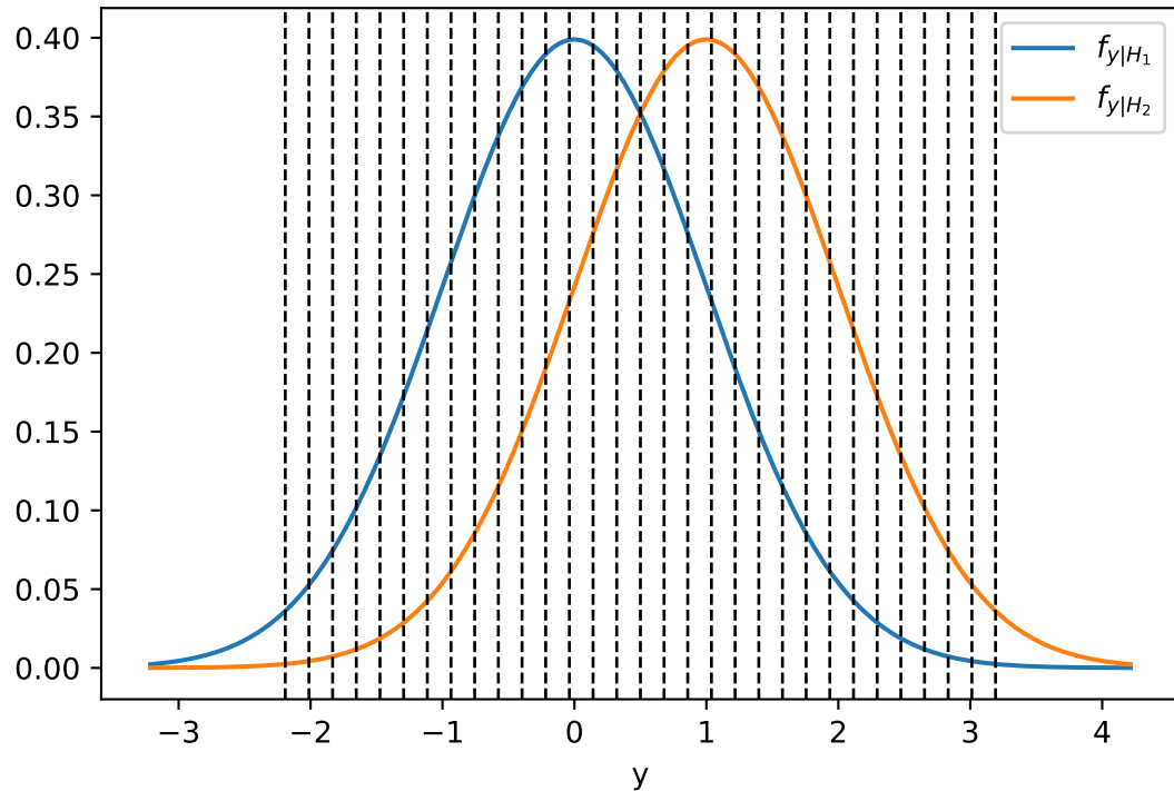
Setup A (vanilla), \Delta^* = 0.1794
