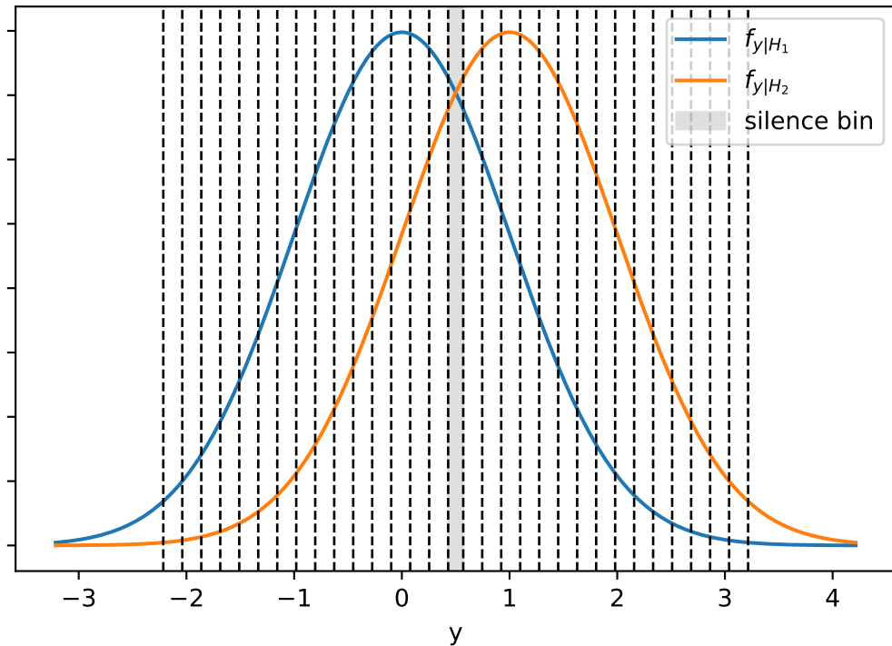
Setup B (silence), \Delta^* = 0.1763 , \delta^* = 0.0699
