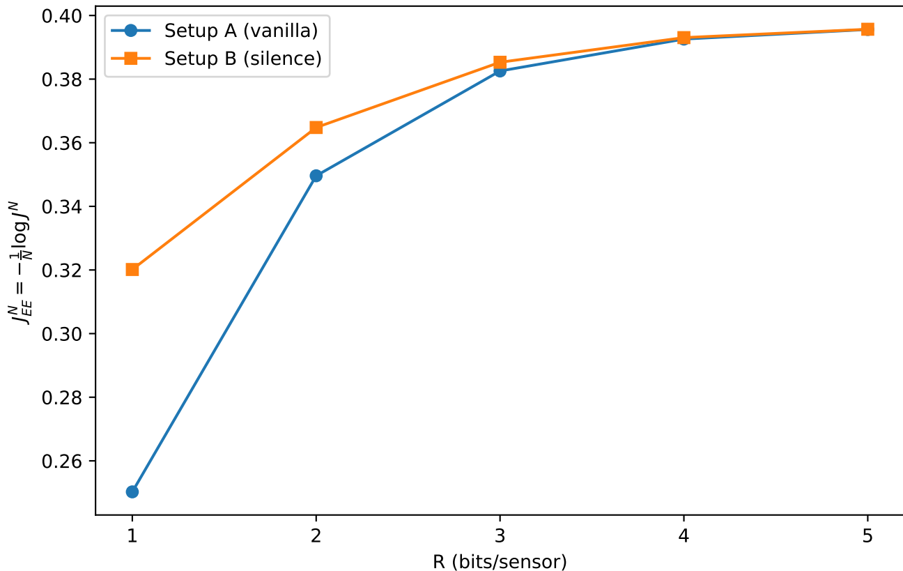
Normalized error exponent at optimal ( \Delta^* , \delta^* ) N=3000, SNR=+5dB ( \mu=1.778 , \sigma=1 )
