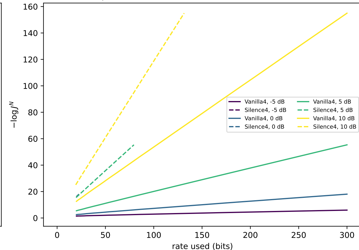
Error exponent vs. R (solid = Vanilla4, dashed = Silence4)
