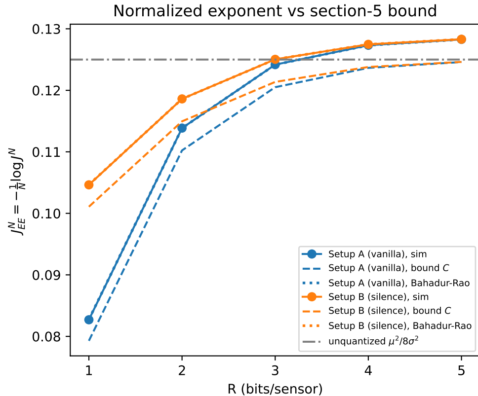
Simulation 2 at optimal (\Delta^*, \delta^*) : N=1000, SNR=0dB ( \mu=1 , \sigma=1 ), method=tilted
