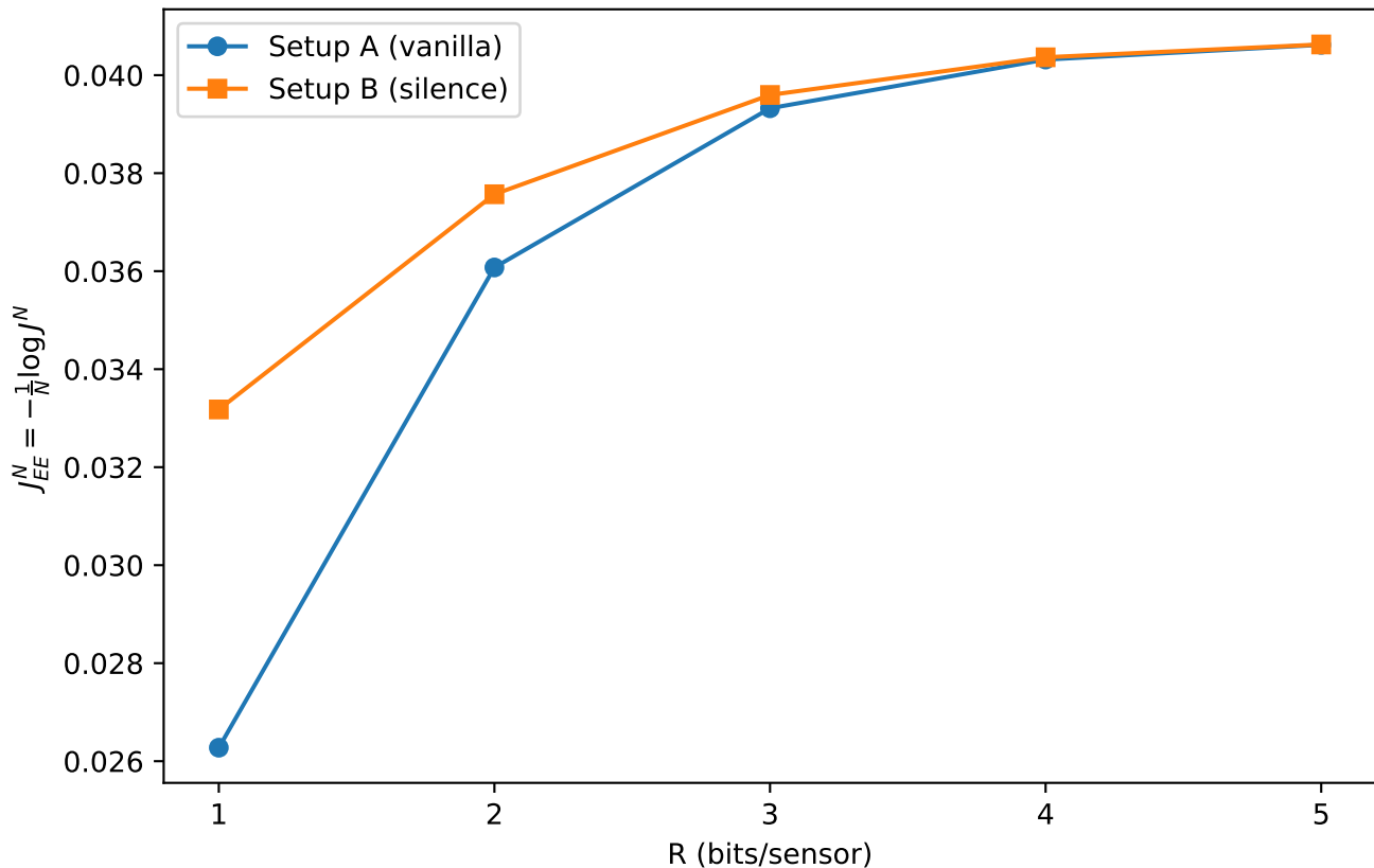
Normalized error exponent at optimal ( \Delta^*, \delta^* ) N=3000, SNR=-5dB ( \mu=0.5623 , \sigma=1 )
