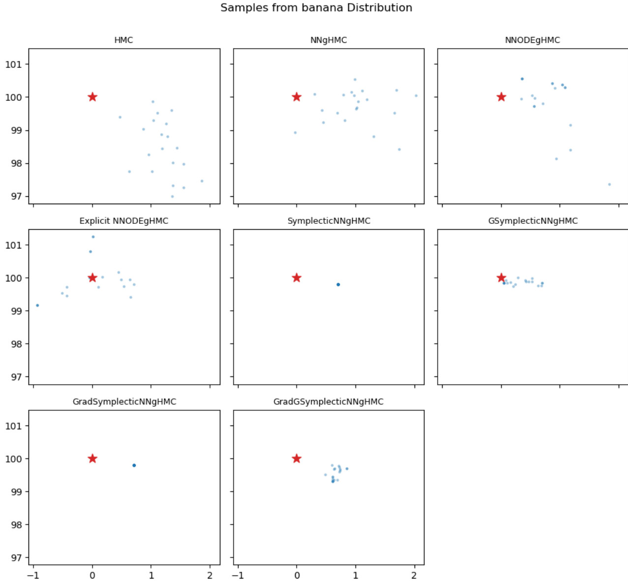
Figure 4. Samples from each method for the Banana distribution. This target should not be read as a comparison between methods: exact HMC itself attains an effective sample size of order 1 here at L = 5 , \epsilon = 0.1 , so no method is sampling it adequately. The banana’s curvature grows with \theta_1 , which caps the stable step size while the marginal scale demands long trajectories — a conditioning problem that a fixed identity mass matrix cannot resolve, and one better addressed by the Riemannian methods of Section 3.4.
