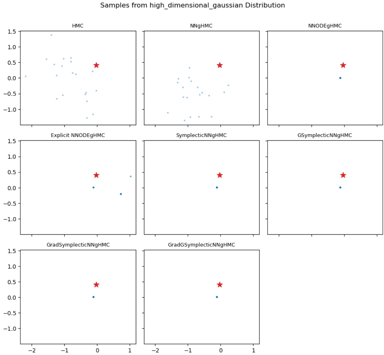
Figure 5. Samples from each method for the 30-dimensional Gaussian (first two coordinates shown).
