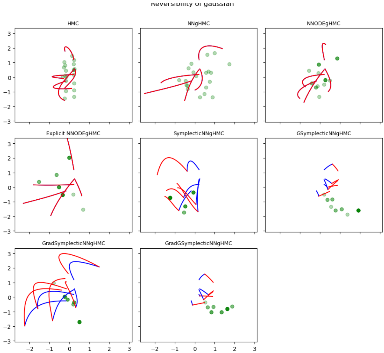
Figure 3. Reversibility of the Hamiltonian paths for the multivariate Gaussian: forward trajectories (blue) and the paths obtained by flipping the momentum and integrating back (red), over the sampled positions (green). Quantitative values for every target are given in Figure 10. Note that the unsymmetrized symplectic networks sample a split support, so their backward paths start from a region the target does not concentrate on.
