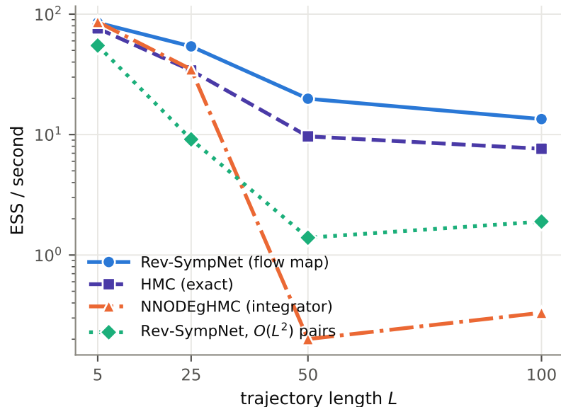
(b) Cost scaling with trajectory length
