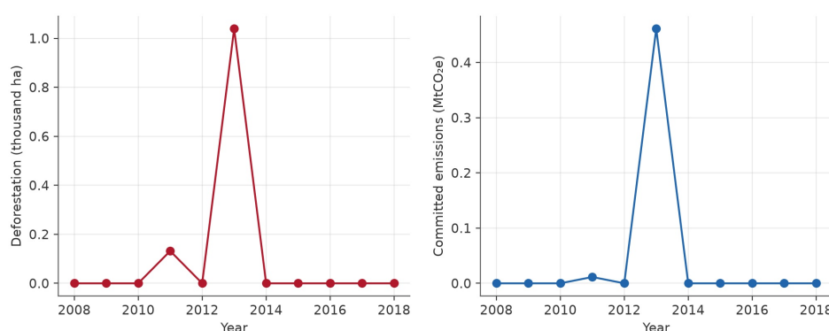
Figure S2. Annual synthetic deforestation and committed carbon emissions inside the signatory direct zone.
