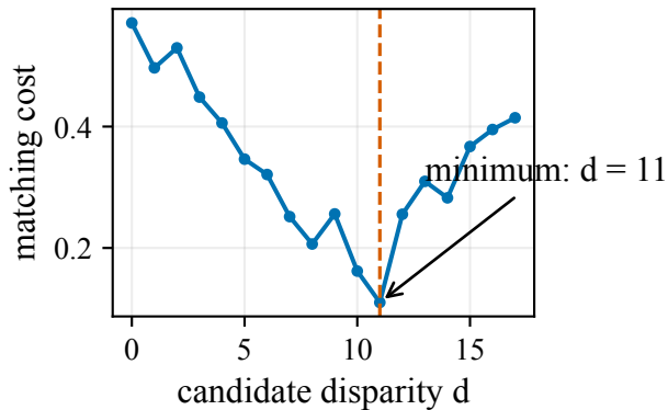
(c) Cost profile for one pixel
