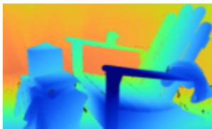
Ground truth
