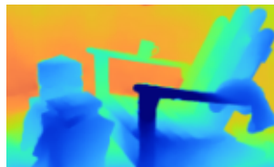
Prediction
