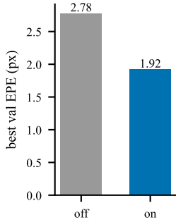
(a) augmentation
