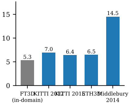
bad-2 (%)
