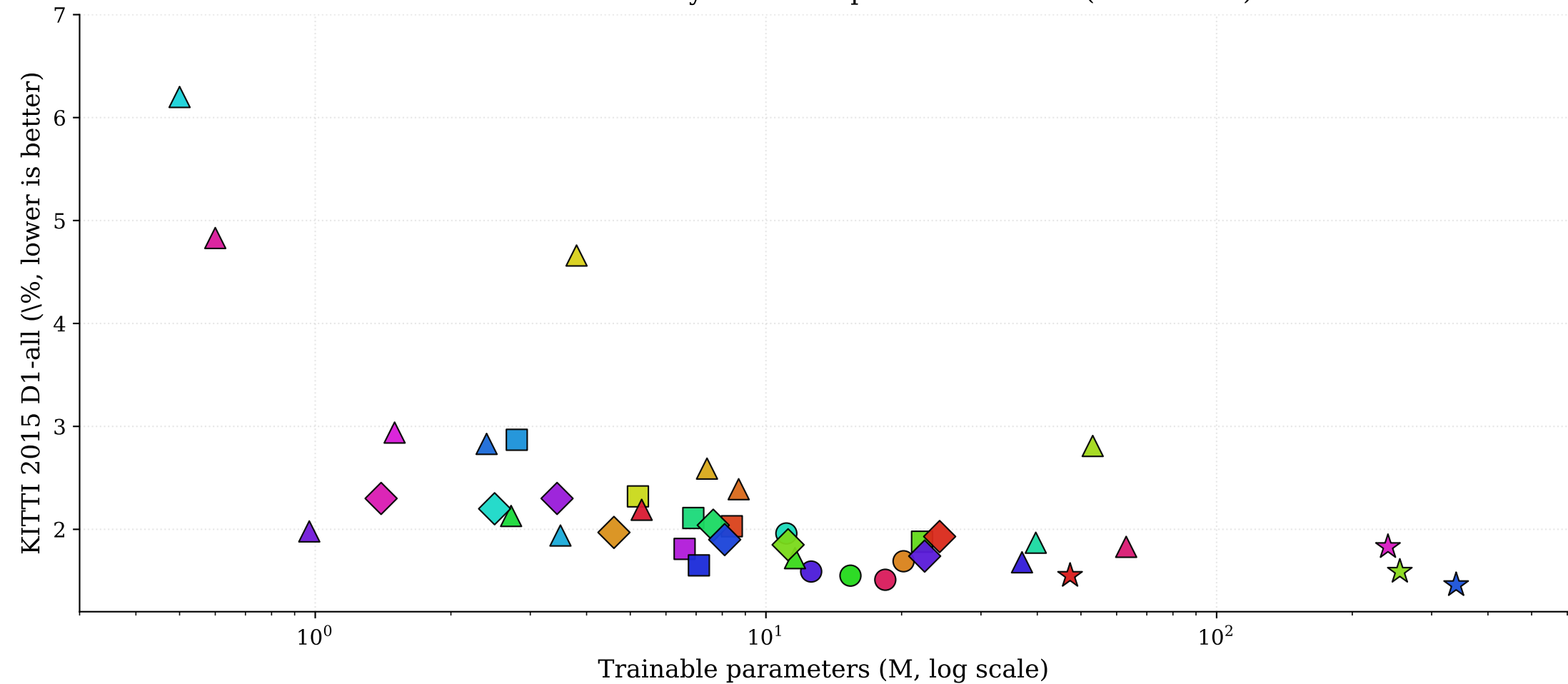
Model size vs. accuracy across deep stereo methods (2017--2026)
