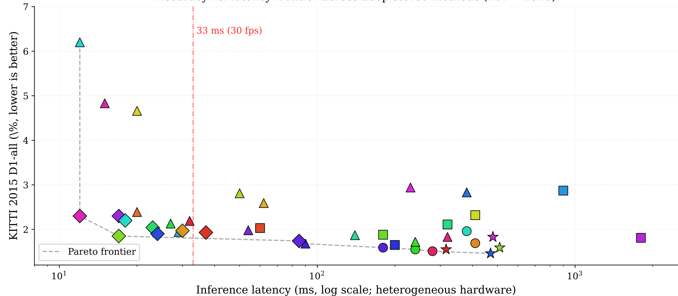
Accuracy vs. latency frontier across deep stereo methods (2017--2026)
