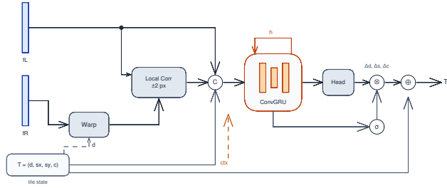
Fig. 3. One recurrent refinement iteration. The right features are warped by the current disparity, a five-offset local correlation is evaluated around it, and the concatenated input of (3) drives the convolutional GRU of (4); a gated head emits residuals for the disparity, the two plane slopes, and the confidence.
