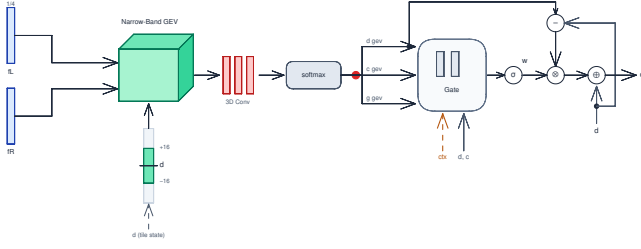
Fig. 4. Narrow-band geometry volume and fail-soft fusion. Thirty-three hypotheses in a \pm 16 band around the tile disparity are regularized and read out by (6); the gate of (7) blends the proposal into the tile estimate with a weight that starts near zero.
