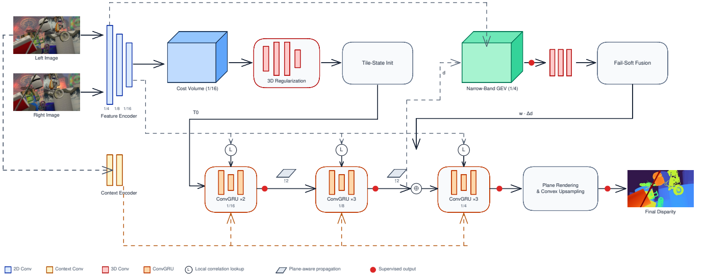
Fig. 2. StereoLite architecture. (1) A shared truncated YOLO26s encoder processes both views and a separate 32-channel context encoder reads the left image alone. (2) A group-wise cost volume at one sixteenth resolution, regularized by a small three-dimensional CNN, seeds the tile state T = (d, s_x, s_y, h, c) by soft-argmax. (3) Convolutional GRU updates refine the state over two, three, and three iterations at one sixteenth, one eighth, and one quarter resolution, with plane-aware propagation between scales. (4) A narrow-band geometry encoding volume at quarter resolution proposes an independent disparity that a learned fail-soft gate blends into the tile estimate. (5) Plane rendering and two learned convex upsampling stages produce the full-resolution disparity. Red dots mark the supervised outputs of the multi-scale objective.
