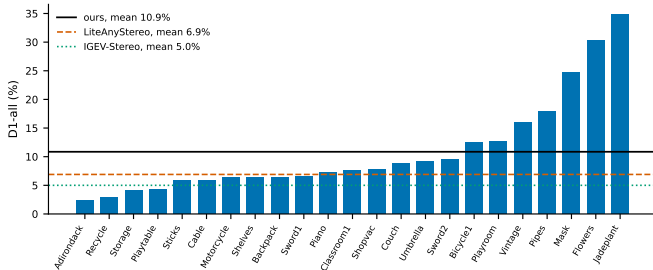
Fig. 8. Per-scene zero-shot D1-all on Middlebury 2014, sorted by error. Sixteen of the 23 scenes fall below 10 percent; four scenes with dense thin repeated structure and near-cap disparities raise the mean to 10.9 percent.
