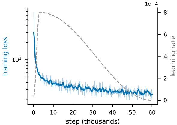
(a) loss and OneCycle schedule
