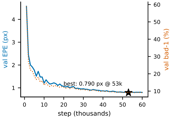
(b) held-out validation (400 pairs, native axis)
