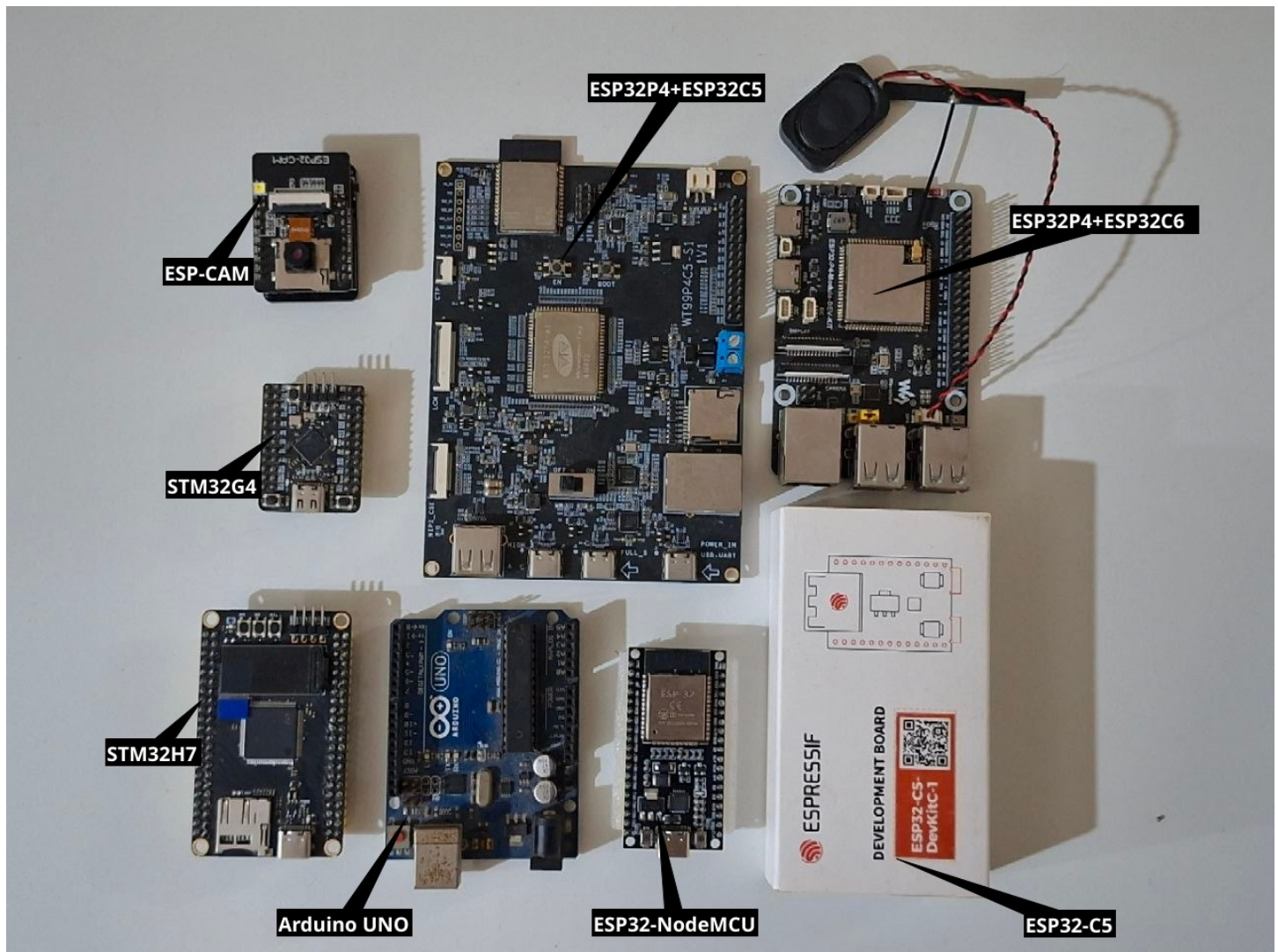
Microcontroller development boards used for firmware and peripheral driver work.
