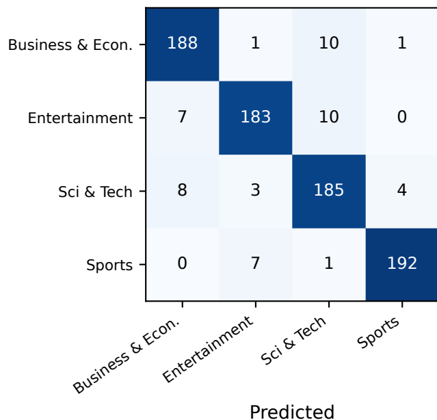
TF-IDF + LinearSVC (acc 0.935)
