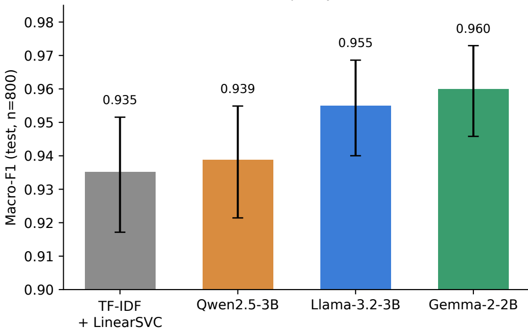
Macro-F1 with 95% bootstrap CI (y-axis truncated at 0.90)
