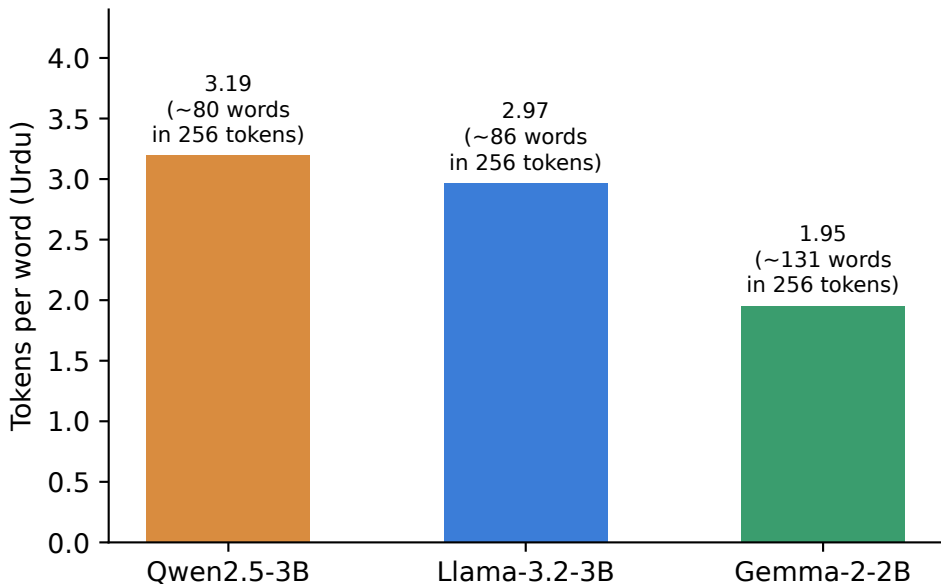
Tokenizer fertility on Urdu training text
