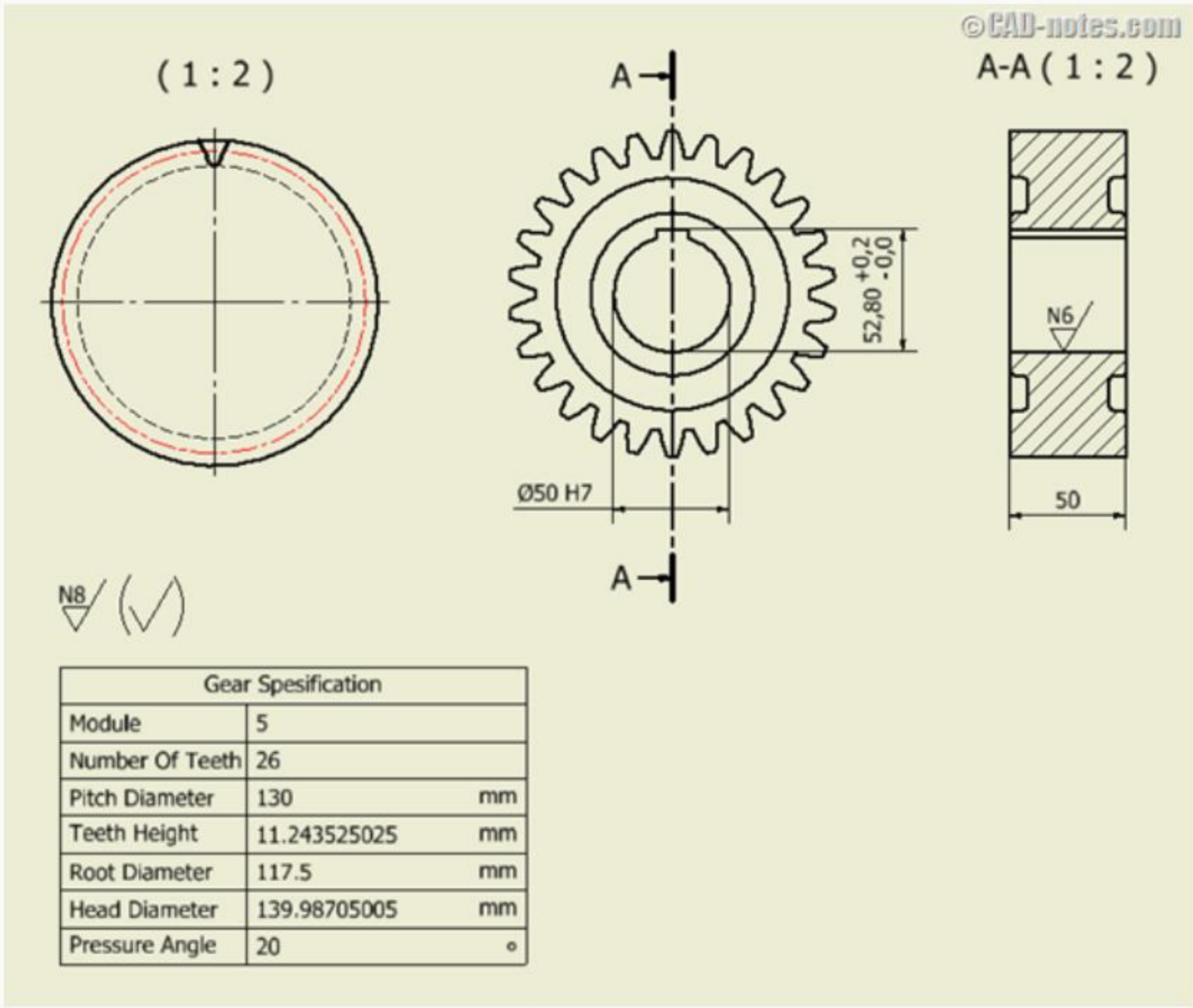
Machining Tolerances & Specification Tables
