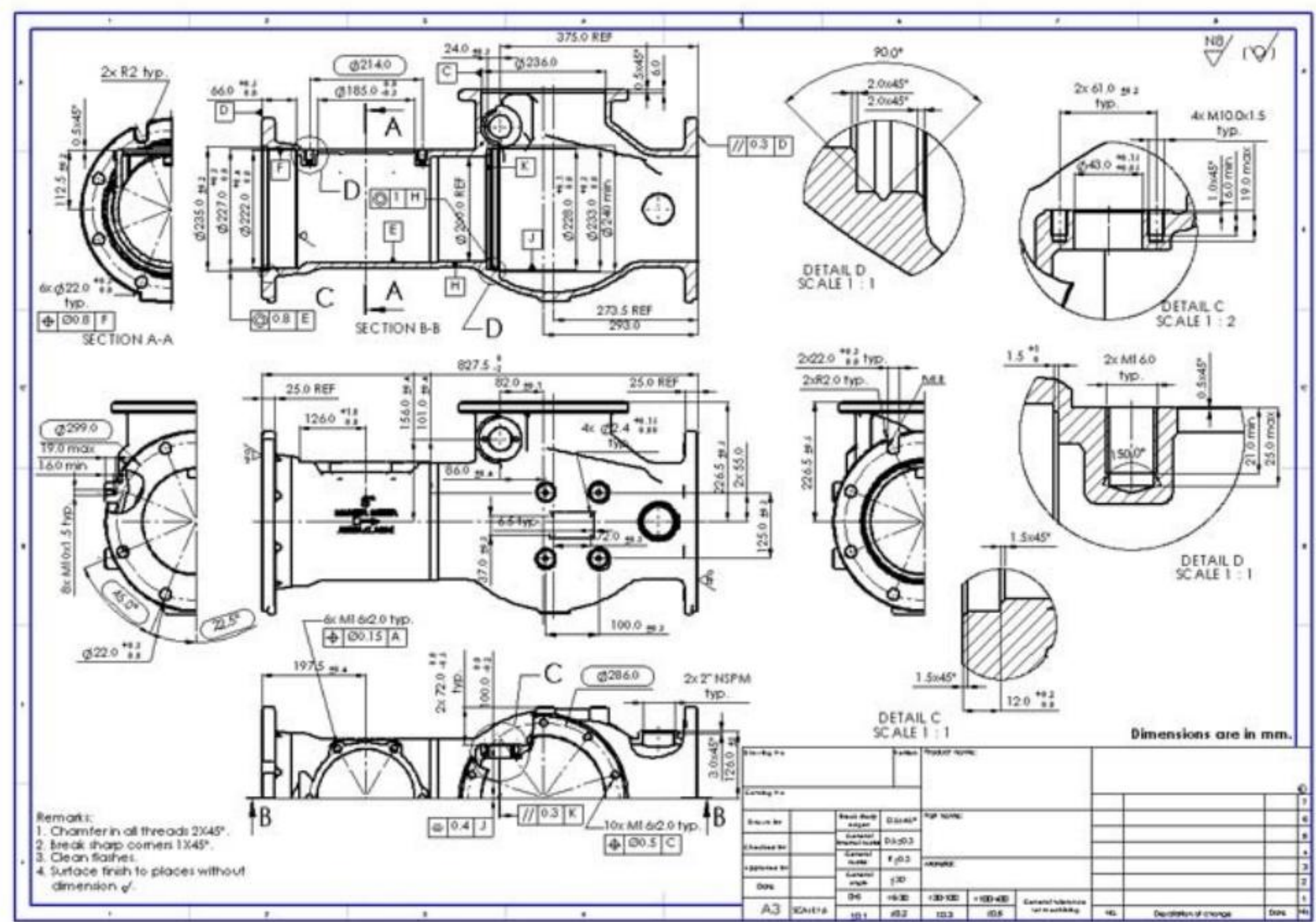
Casing Blueprint with Full GD&T
