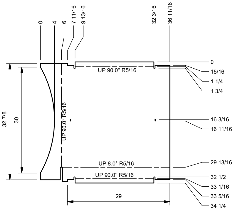
FLAT SCALE 1/16
