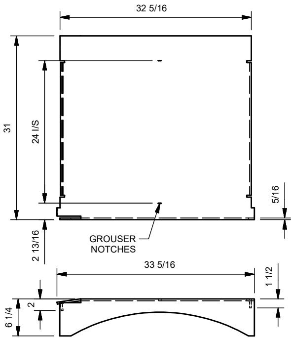
ELEVATION SCALE 1/16
