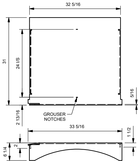
ELEVATION SCALE 1/16
