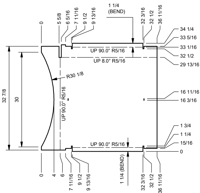
FLAT PATTERN SCALE 1/16
