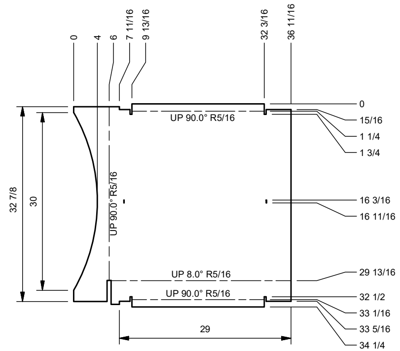
FLAT SCALE 1/16
