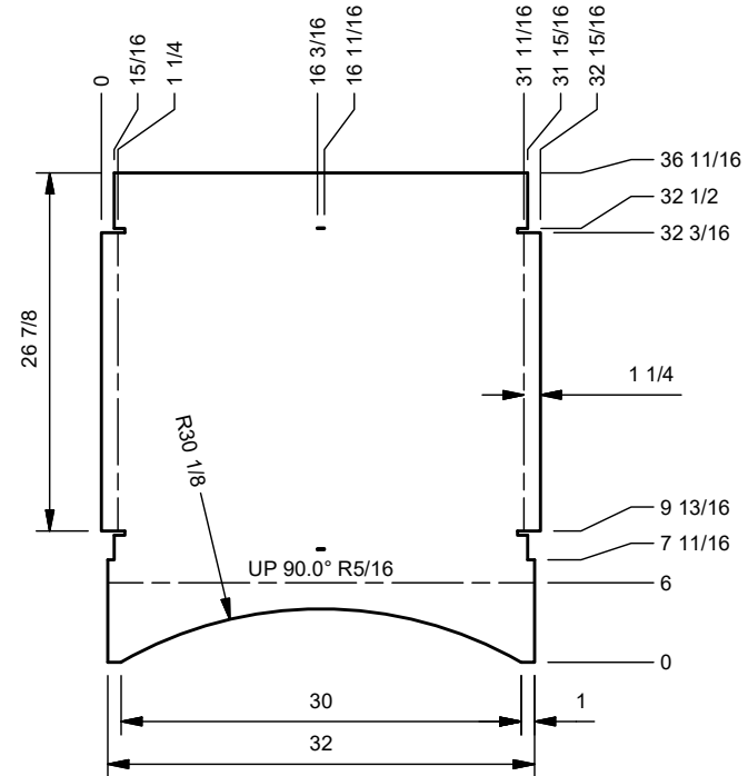
FLAT PATTERN SCALE 1/16
