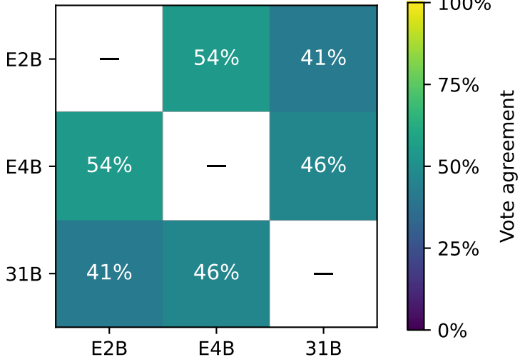
Greedy
