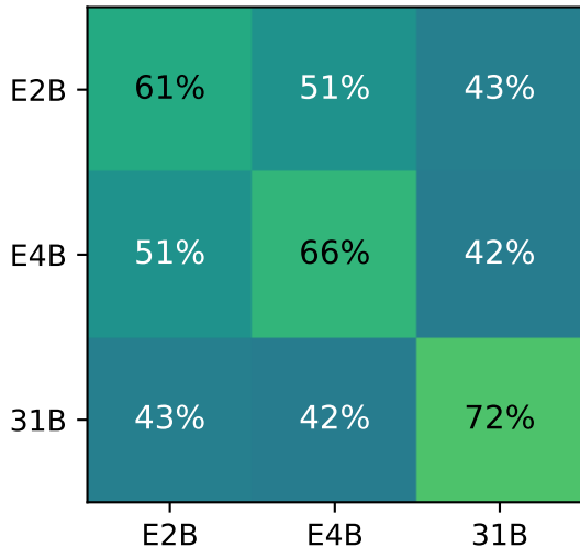
Stochastic
