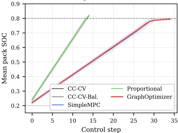
(a) Mean SOC trajectories \pm 1\sigma — LFP, N=30
