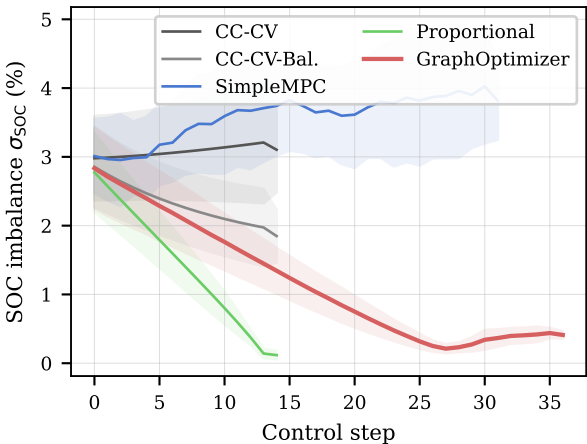
(b) SOC imbalance evolution — LFP, N=30
