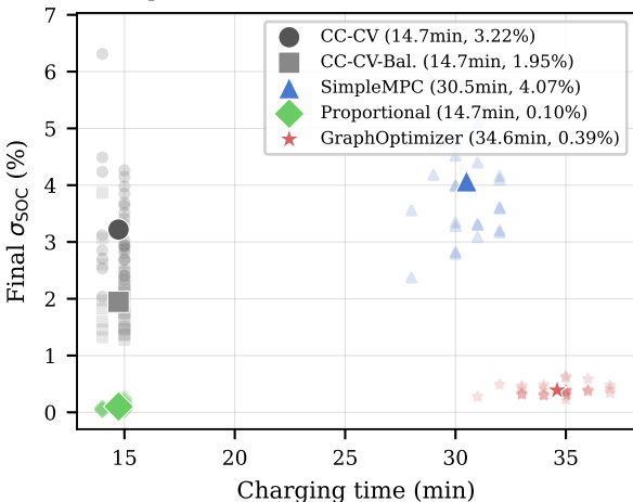
Speed-balance trade-off — LFP, N=30
