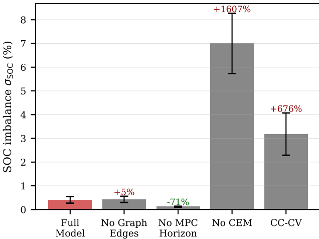
(a) SOC imbalance by ablation
