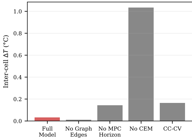
(b) Thermal gradient by ablation
