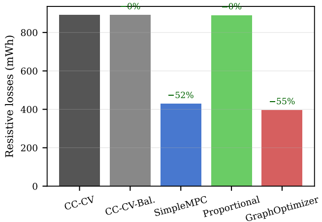
(b) Resistive losses
