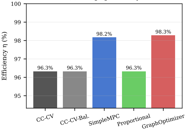
(a) Charging efficiency
