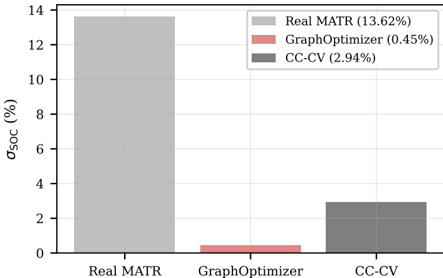
(a) SOC imbalance — MATR replay
