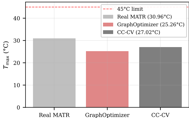
(b) Peak temperature — MATR replay
