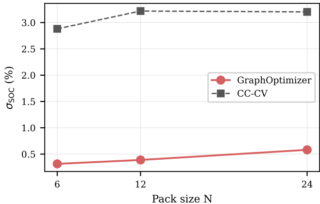
(b) SOC imbalance vs pack size
