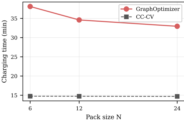
(a) Charging time vs pack size
