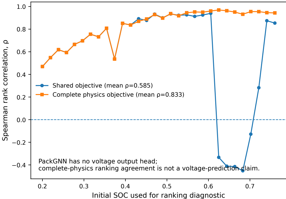
PackGNN v2 candidate-ranking fidelity
